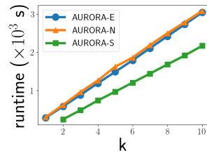
Fig. 12: running time vs. number of k on Pokec dataset
